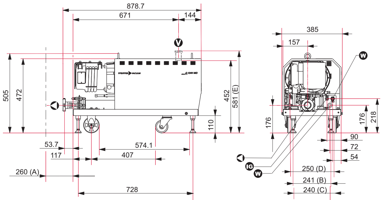
Fig. 12: A124H MD - Dimensions in mm
