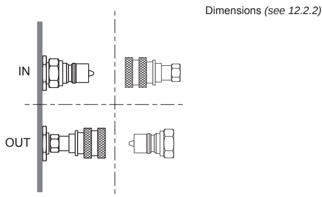
Fig. 5: Water circuit connection
