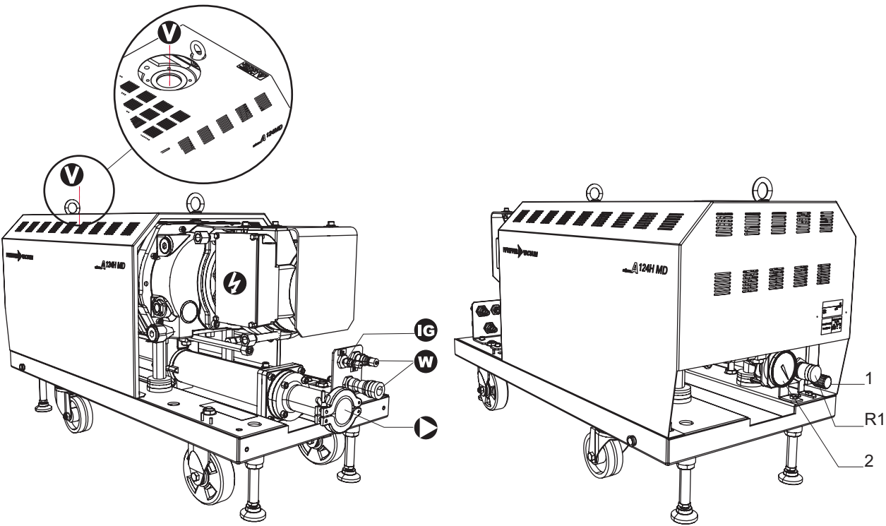
Fig. 2: Man/machine interfaces
