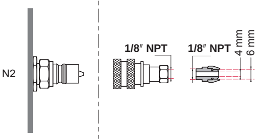
Fig. 7: Nitrogen circuit connection
