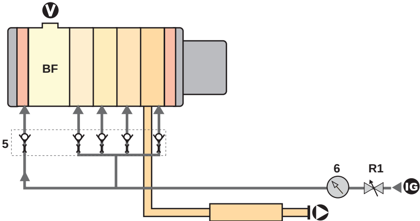
Fig. 8: Nitrogen injection device
