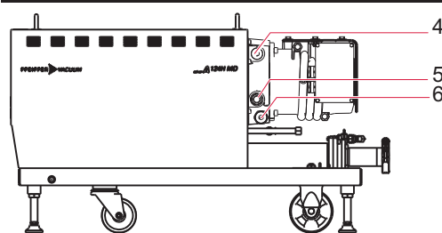
Fig. 3: Oil case filling
