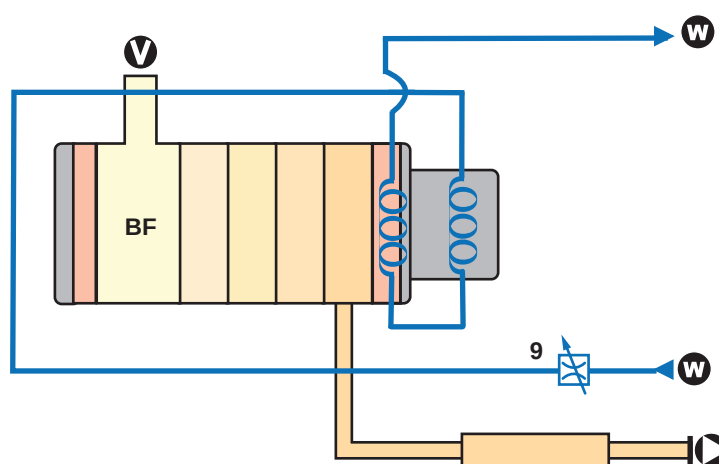
Fig. 6: Water circuit device
