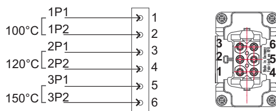
Fig. 11: Connecting of the thermal safeties cable
