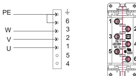
Fig. 10: Cabling of the power supply connector
